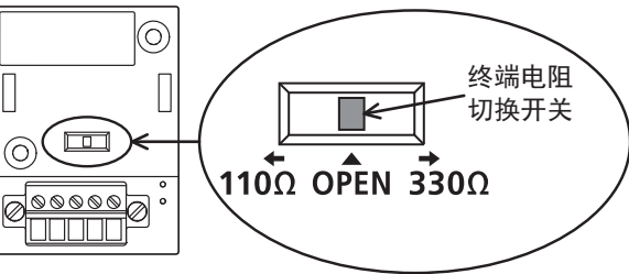
■FX5-485-BD
