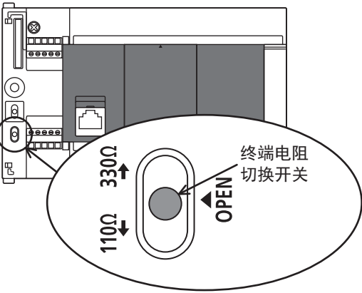
■FX5-485-BD
