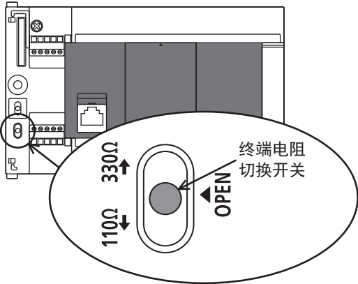
■FX5-485-BD
