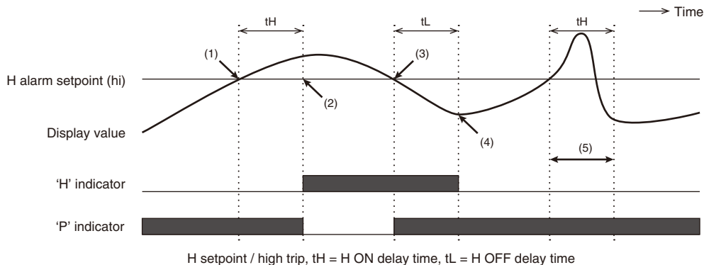
Figure 1: Example of high alarm trip and indicators action with ON/OFF delay time
